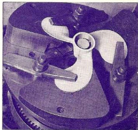
Boring a propeller by the Pitch Block Method
