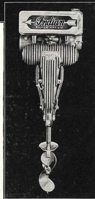
Above: Note the clean, compact, design of the Silver Arrow Motor, and the absence of small parts. Simplicity and stamina are built into this design. The spacious muffler, cast in one single piece of aluminum alloy, is well finned for cooling.
