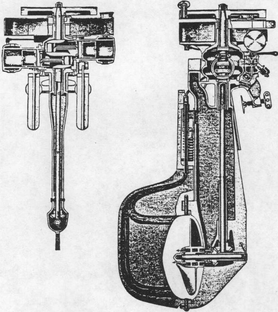
Sectional Views of Elto Light Twin
