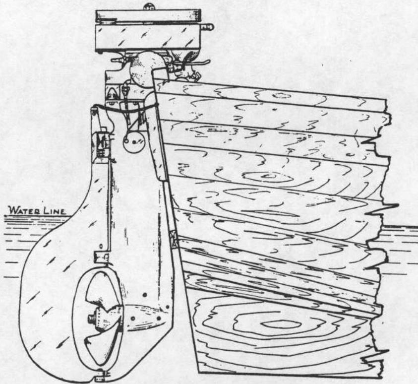
Fig. 13 (Side View)
