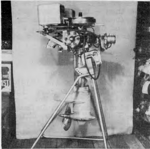
ELTO RACING SUPER C 30 CUBIC INCH TWIN BATTERY IGNITION
