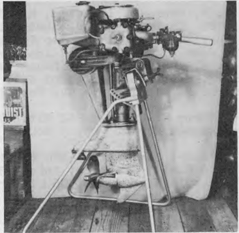
1932 CROSS 4 CYCLE SEA GULL 30 CUBIC INCH TWIN
